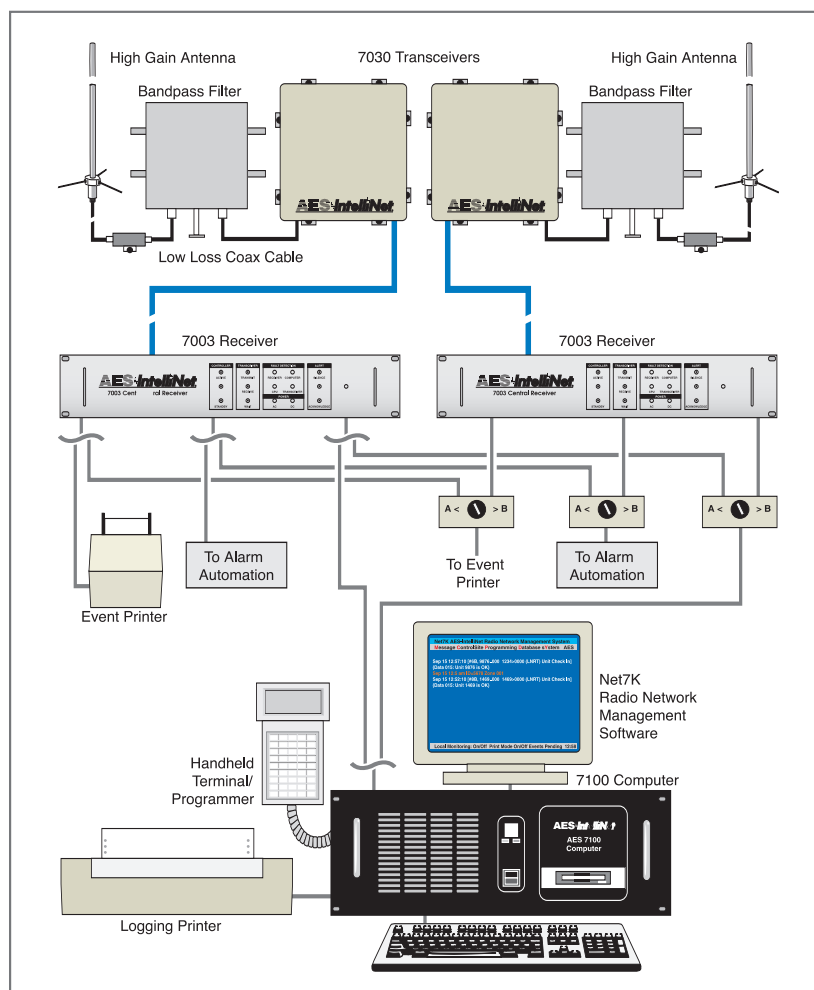
7003 Dual Redundant Configuration – one primary, one backup
