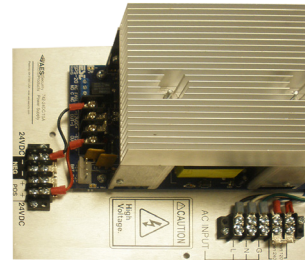
742 10A Power Supply Retrofit Kit
